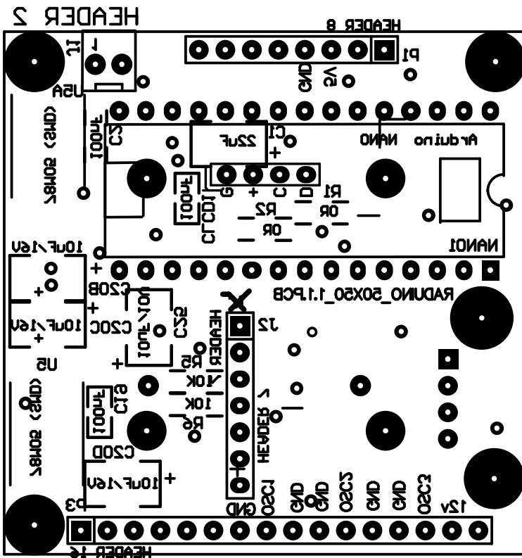
REF: RADUINO_50X50_1.sch
