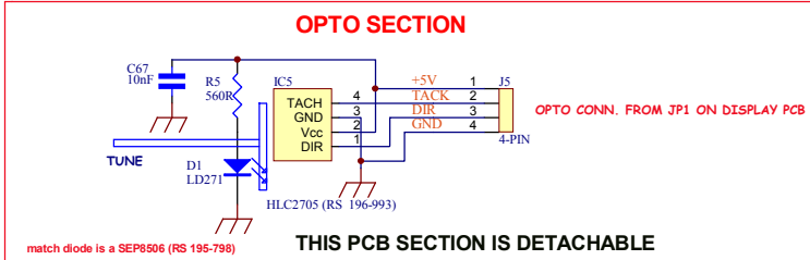
BUTLER OSC, DDS CARRIER AND AMP PCB
