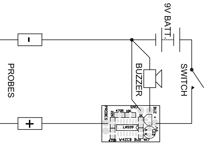
LOW VOLTAGE CONTINUITY TESTER
